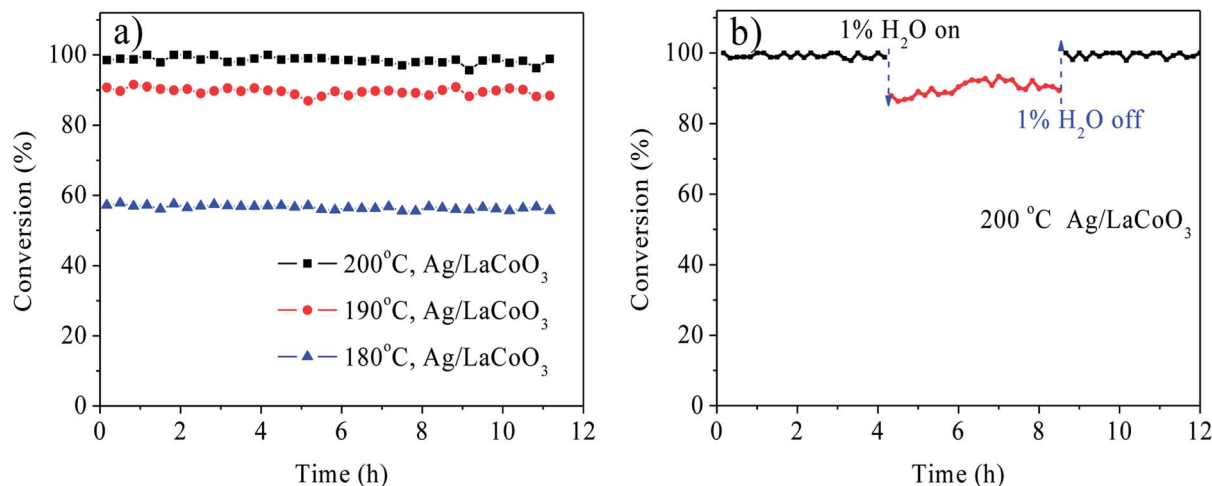
Fig. 6 The stability of ethyl acetate over Ag/LaCoO 3 at 180, 190 and 200 °C (a), effect of water vapor on on-stream reaction over Ag/LaCoO 3 (b). Ethyl acetate concentration: 500 ppm; ethyl acetate/O 2 molar ratio: 1/400; WHSV: 60 000 mL (g h) -1 .
