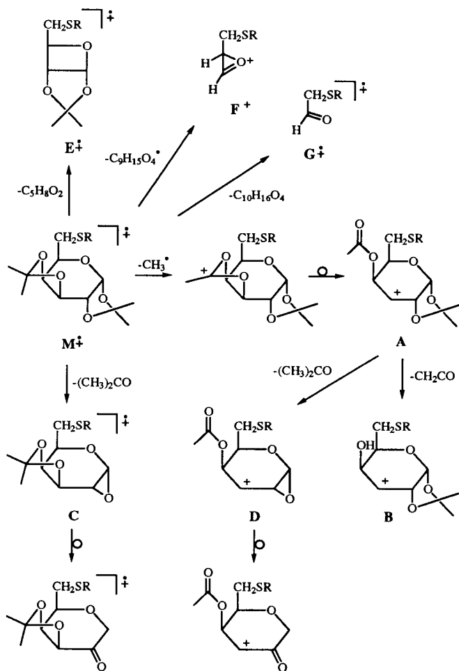
Scheme 3
