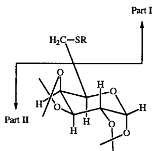
Scheme 2
