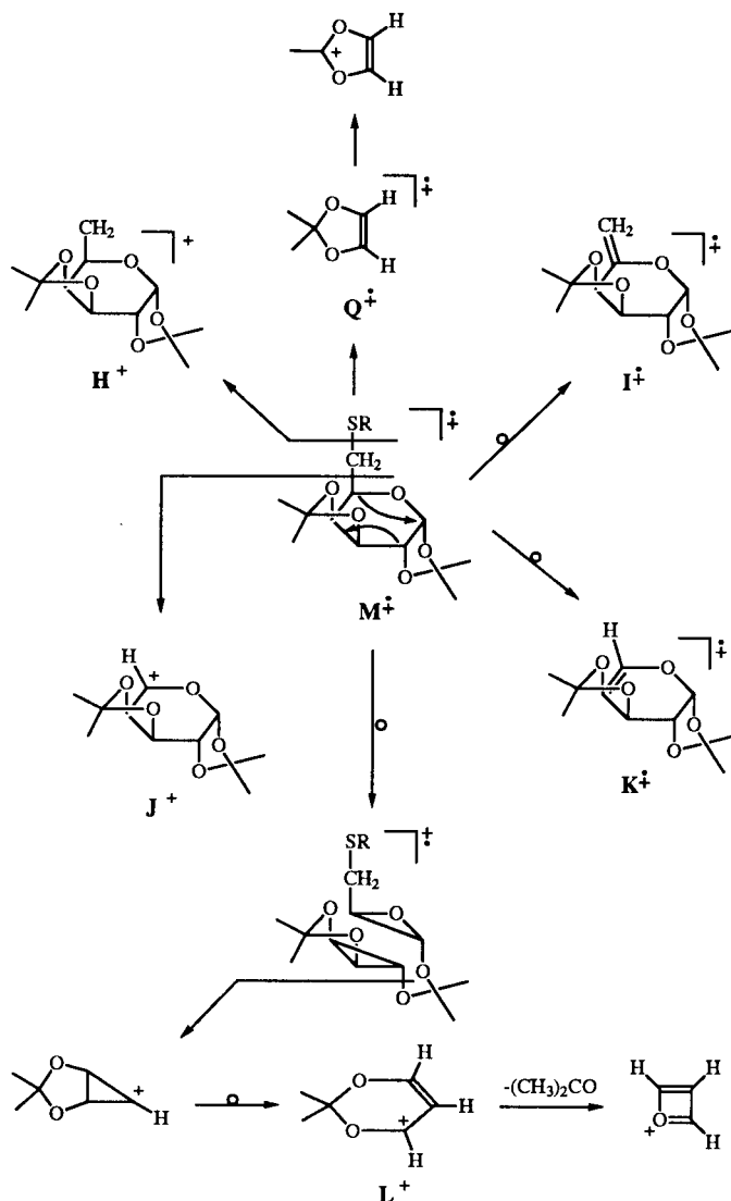
Scheme 4
