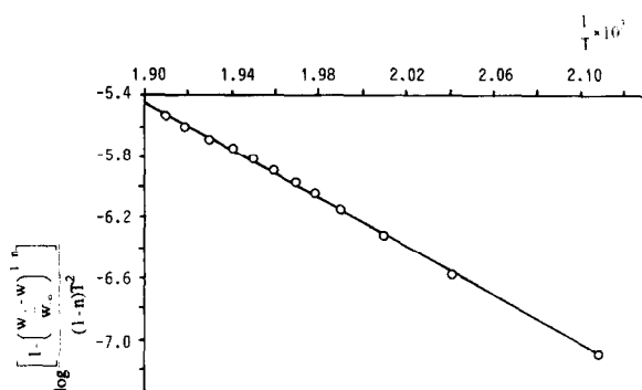
Fig. 5. Coats-Redfern plot for [\text{Pd}(\text{S}_2\text{CNHCx})_2] .
