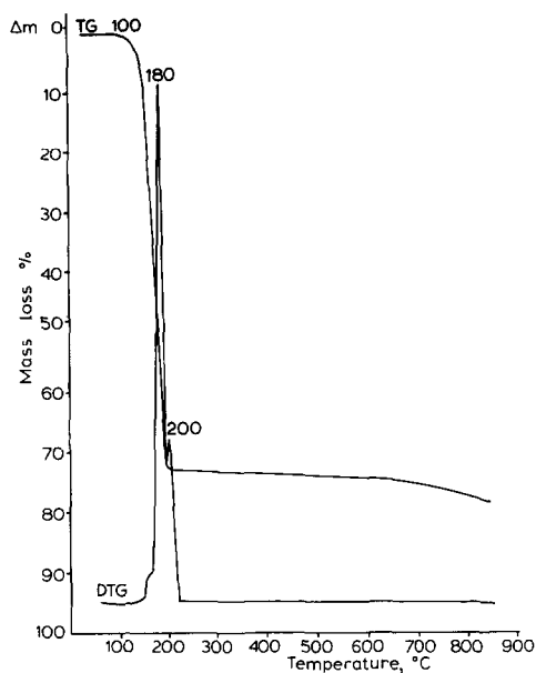
Fig. 1. Thermoanalytical curves of [\text{Ni}(\text{S}_2\text{CNHBu}'')_2] in nitrogen.
