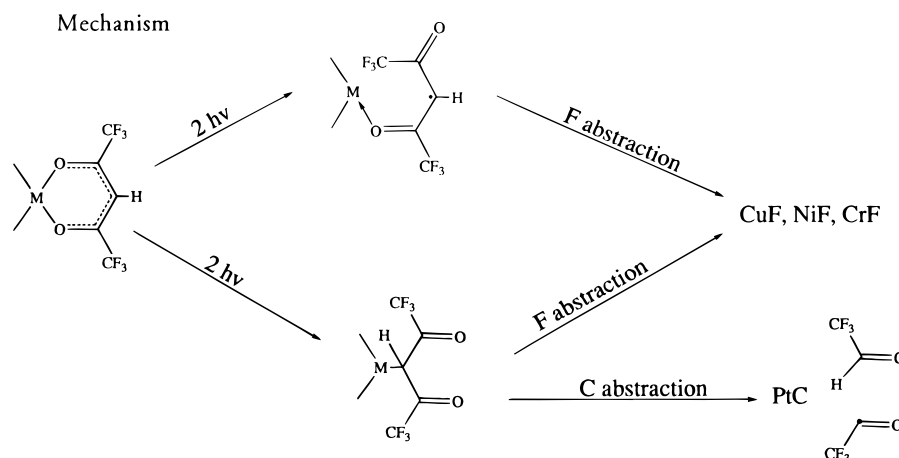
Figure 5. Proposed intramolecular rearrangements that explain the observed photofragmentation patterns of the metal–hfac compounds studied.
