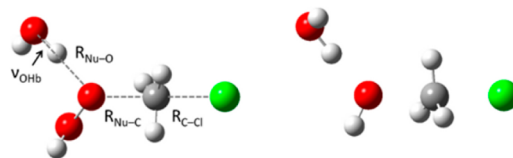
Figure 7. Transition-state structures for the \text{S}_{\text{N}}2 reaction of the microsolvated anions \text{HOO}^-(\text{H}_2\text{O}) and \text{HO}^-(\text{H}_2\text{O}) with methyl chloride optimized at the MP2/6-311++G(d,p) level of theory. The bond lengths R_{\text{Nu}-\text{C}} , R_{\text{C}-\text{Cl}} , and R_{\text{Nu}-\text{O}} , and the vibrational frequencies of the hydrogen-bonded OH stretch, \nu_{\text{OHb}} , are found in Table 3 for all anions.
