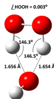
Figure 3. Lowest-energy structure of the microsolvated anion \text{HOO}^-(\text{H}_2\text{O}) optimized at the CCSD(T)/aug-cc-pVTZ level of theory.
