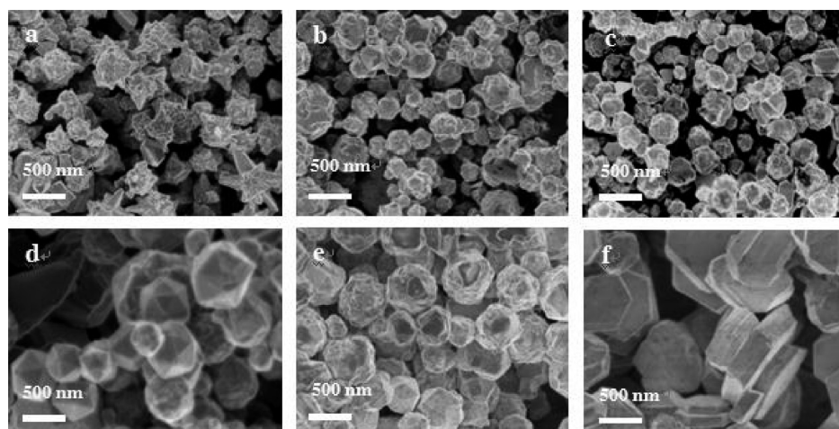
Figure 5. SEM images of NiCo NCs in different compositions: (a, b) Ni and \text{Ni}_{82}\text{Co}_{18} multi-horn-sphere, (c) \text{Ni}_{76}\text{Co}_{24} irregular polyhedral NCs, (d) \text{Ni}_{48}\text{Co}_{52} icosahedral NCs, (e) \text{Ni}_{25}\text{Co}_{75} truncation icosahedral NCs, (f) \text{Ni}_{16}\text{Co}_{84} nanoplates.
