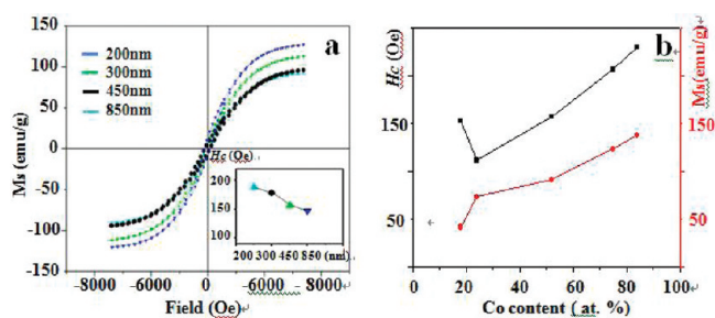
Figure 7. Magnetic behavior of icosahedral NiCo NCs measured at 300 K: (a) M – H curves for 200, 300, 450, and 850 nm sized icosahedral NCs with inset curve of H_c over the particle size. (b) The variation of M_s and H_c for NiCo NCs within different compositions.
