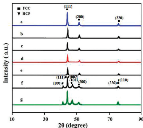
Figure 3. XRD patterns of NiCo nanocrystals in different compositions: (a) Ni, (b) \text{Ni}_{82}\text{Co}_{18} , (c) \text{Ni}_{76}\text{Co}_{24} , (d) \text{Ni}_{48}\text{Co}_{52} , (e) \text{Ni}_{25}\text{Co}_{75} , (f) \text{Ni}_{16}\text{Co}_{84} , (g) Co.
