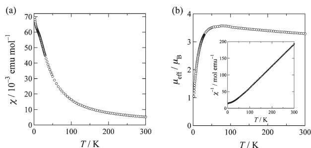
Figure 4. Temperature dependence of the magnetic susceptibility (a) and the magnetic moment (b) for TPP[Mn III (Pc)(CN) 2 ] \cdot DCM. The inset shows the reciprocal susceptibility.
