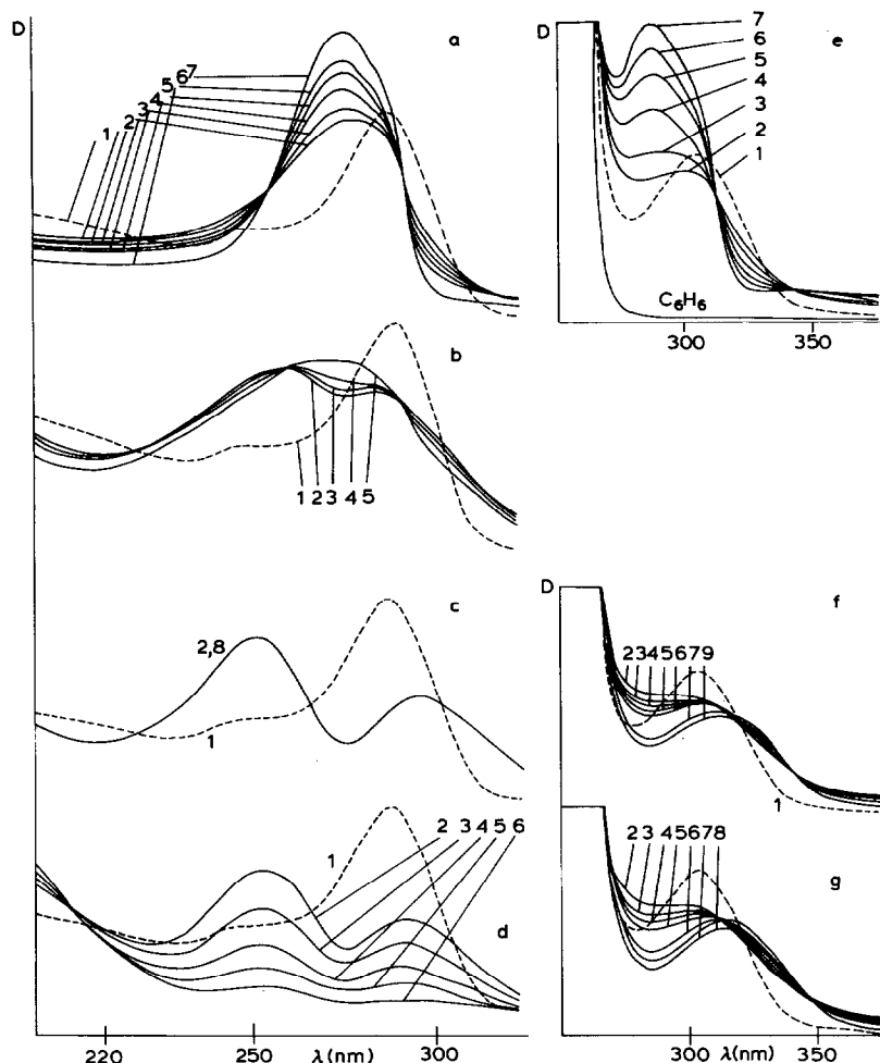
Fig. 3. Absorption spectra of \text{Ni}(\text{acac})_2 (I) and the interaction of \text{Ni}(\text{acac})_2 with \text{AlEt}_3 in cyclohexane at \text{Al}/\text{Ni} = 0.5 (a), 1.5 (b), 2 (c), 15 (d) and in benzene at \text{Al}/\text{Ni} = 1 (e), 2.1 (f), 5 (g) after 3 (2), 10 (3), 30 (4), 60 (5), 120 min (6), 24 hours (7), 3 days (8) and 12 days (9).
