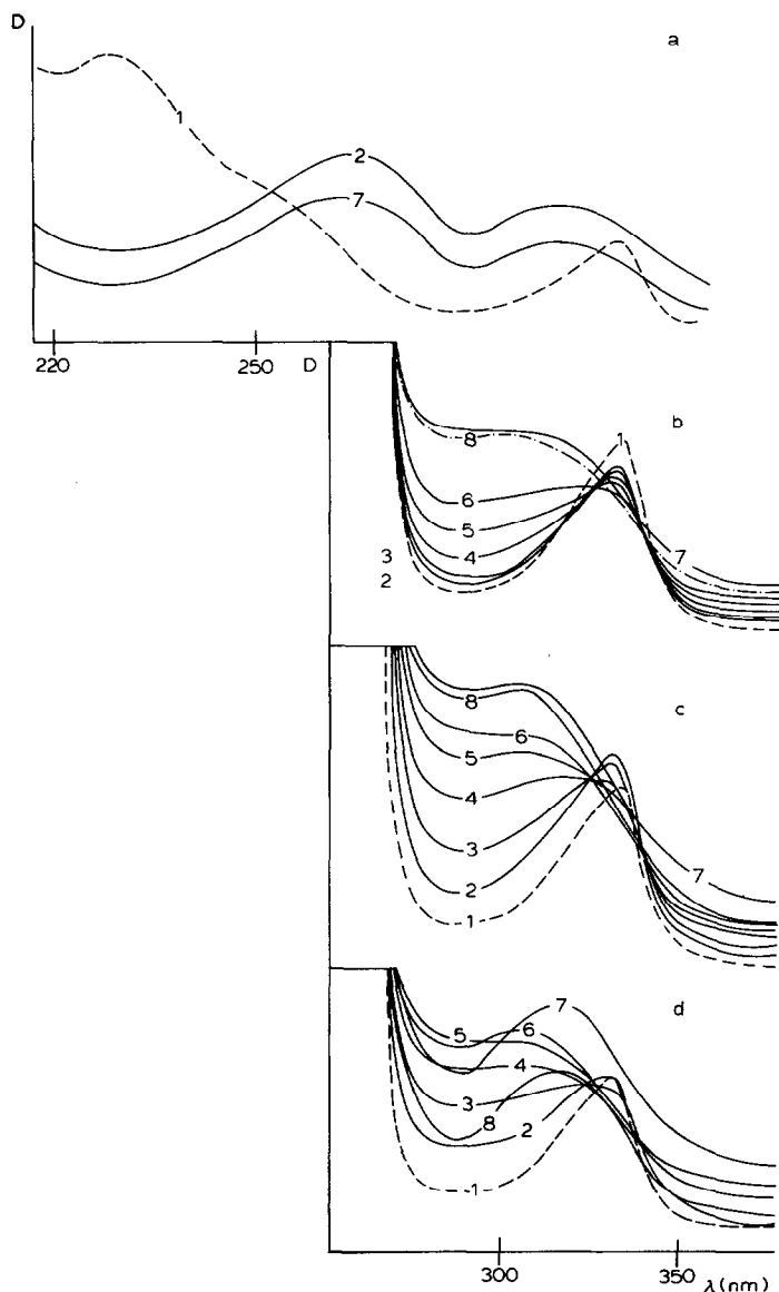
Fig. 6. Absorption spectra of \text{Pd}(\text{acac})_2 (I) and the interaction of \text{Pd}(\text{acac})_2 with \text{AlEt}_3 in cyclohexane at \text{Al/Pd} = 2.1 (a) and in benzene at \text{Al/Pd} = 1.5 (b), 2 (c), 3.7 (d), after 2 (2), 10 (3), 30 (4), 60 (5), 120 min (6), 24 hours (7) and 5 days (8).
