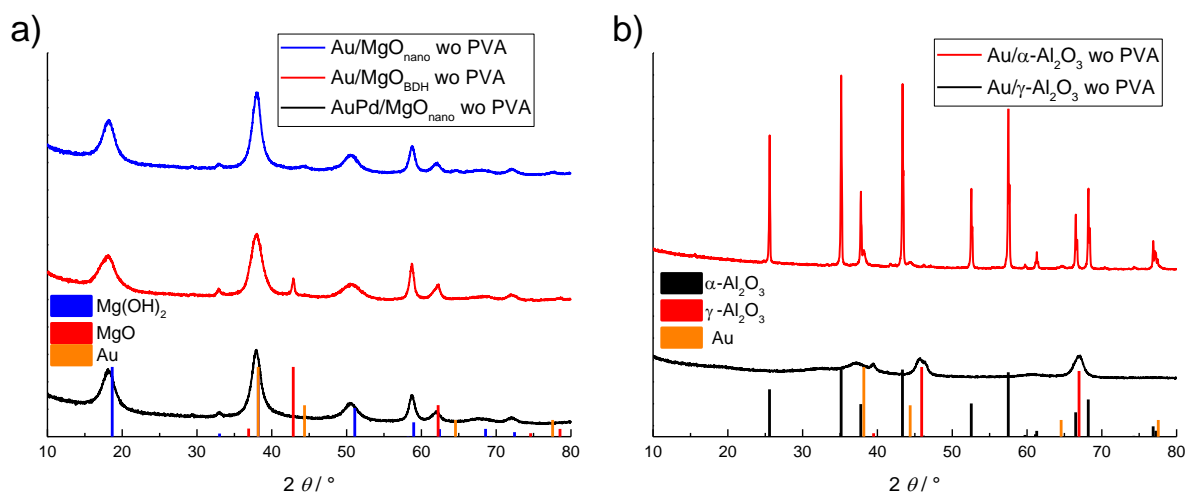
Figure 1. XRD patterns of a) \text{Au}/\text{MgO} and \text{AuPd}/\text{MgO} materials, and b) \text{Au}/\text{Al}_2\text{O}_3 materials. “wo PVA” indicates that no capping agent was used during the catalyst synthesis.
