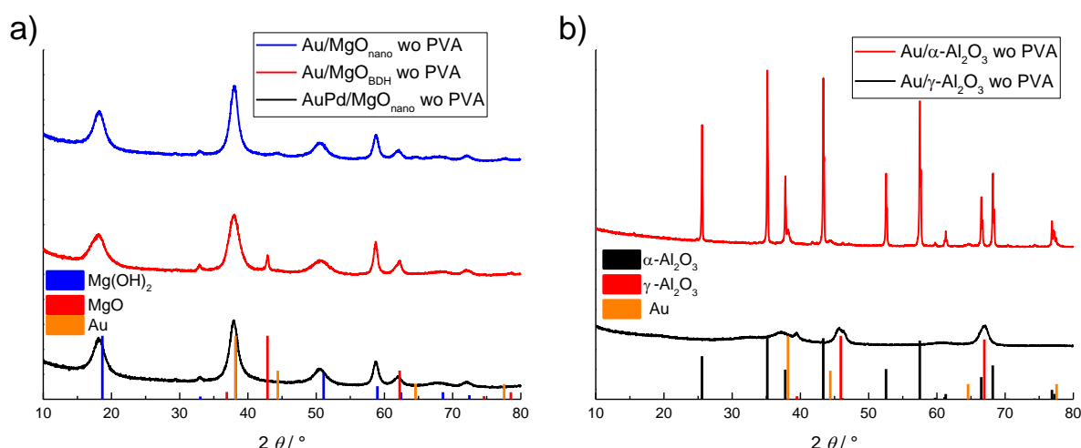
Figure 1a, Au and AuPd NP catalysts supported on MgO mainly consisted of hydrated Mg(OH) 2 , which is due to the aqueous conditions of the sol-immobilisation procedure and is consistent with former reports. [14] The pristine supports prior to noble metal loading showed differing levels of hydration (Supporting Information, Figure S1a and b), which were
