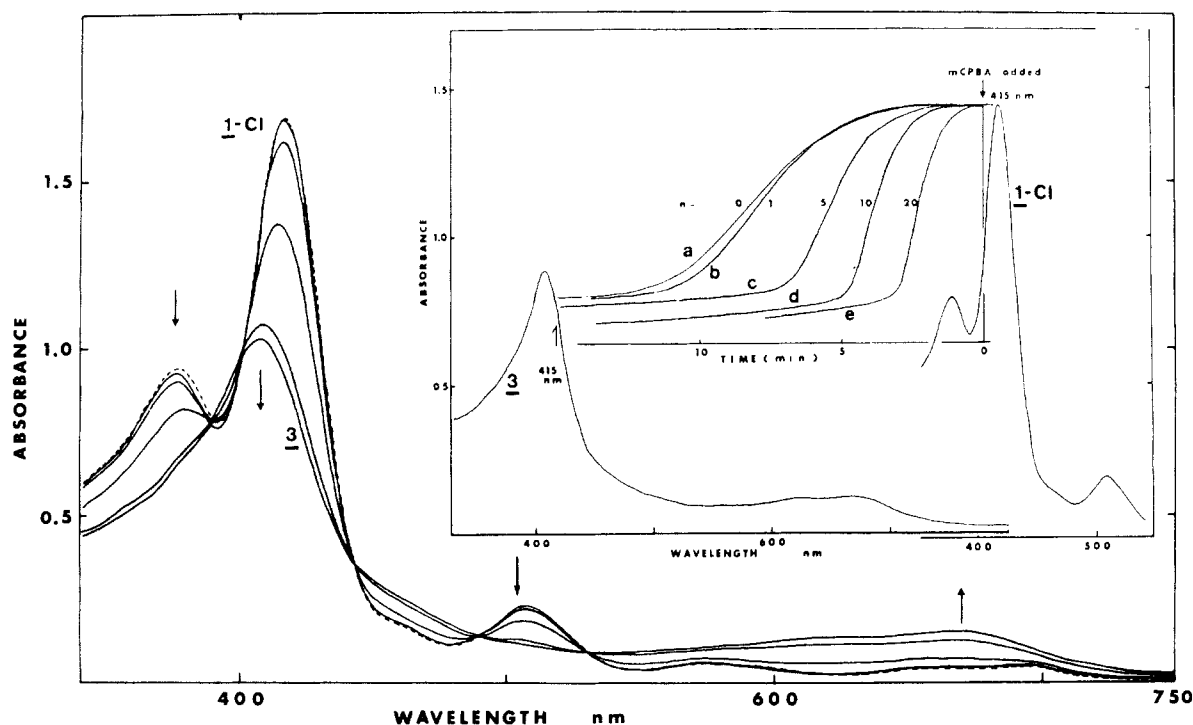
Figure 1. Visible spectral changes upon the addition of 4 equiv of mCPBA to \text{Fe}^{\text{III}}\text{TMP}(\text{Cl}) (1-Cl) [ 1.22 \times 10^{-5} M] (---) in methylene chloride at -46^\circ\text{C} at 2-min intervals (first scan was immediate after the addition of mCPBA). Inset: Effect of acid in the formation of 3. Lines a–e are absorbance changes at 415 nm upon the addition of 3 equiv of mCPBA to the mixture of 1-Cl [ 9.7 \times 10^{-5} M] and n equiv of mCBA in methylene chloride at -46^\circ\text{C} .
