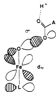
Figure 8. Idealized orbital interaction diagram for acylperoxoiron(III)-L complexes, where L is the sixth ligand to iron.
