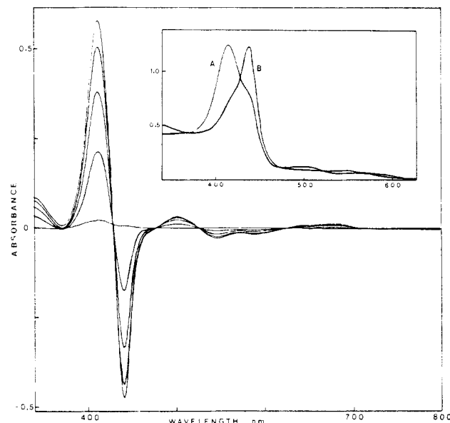
Figure 9. Difference spectral changes in the reaction of 1 -mCB [ 1.27 \times 10^{-5} M] and 0.5 equiv aliquot additions of mCPBA at room temperature in toluene in the presence [sample side] and absence [reference side] of cyclooctene (15 \mu L/3 mL). Inset: After the addition of 2 equiv of mCPBA. A: Sample side. B: Reference side.
