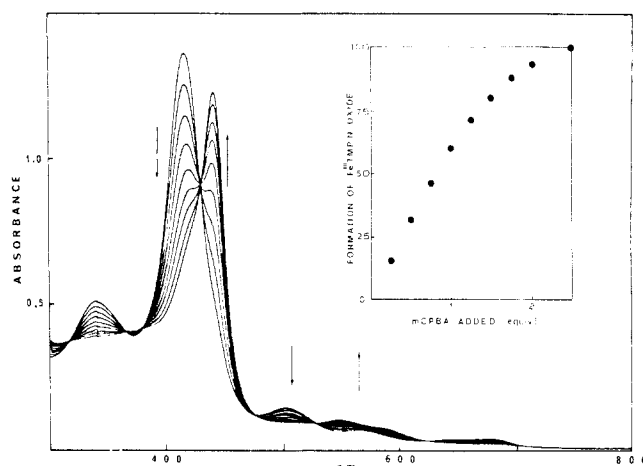
Figure 4. Visible spectral changes upon addition 0.25-equiv aliquots of mCPBA to 1-mCB [ 1.27 \times 10^{-5} \text{ M} ] in toluene at 0^\circ\text{C} .
