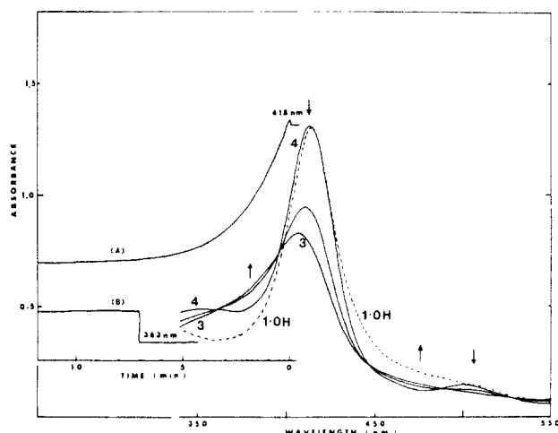
Figure 2. Visible spectral changes for the reaction of 1-OH [ 1.48 \times 10^{-5} M] (---) and 3 equiv of p -nitroperoxybenzoic acid. The spectrum of 4 was recorded immediately after the addition of p -nitroperoxybenzoic acid. Lines labeled A and B represent the time-dependent changes of absorbances at 418 and 363 nm.
