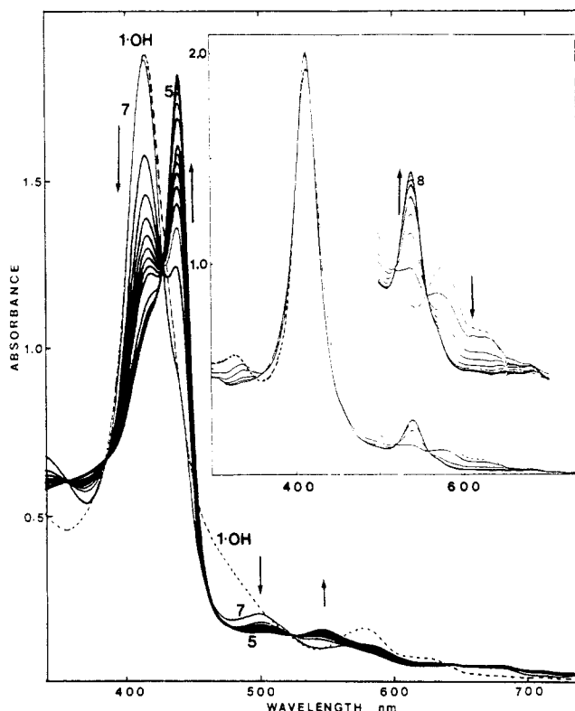
Figure 6. Time-dependent visible spectral changes in the reaction of 1-OH [ 1.7 \times 10^{-5}\text{ M} ] (---) and 3 equiv of mCPBA in toluene at -36^\circ\text{C} . Inset: Same reaction with 3.5 equiv of PPAA at -48^\circ\text{C} .
