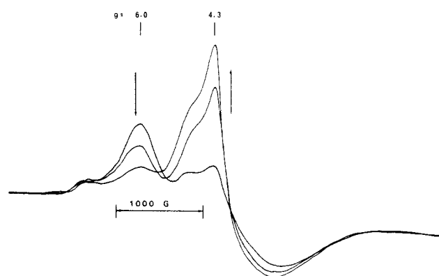
Figure 5. EPR spectral changes for the reaction of 1-mCB and mCPBA in toluene.
