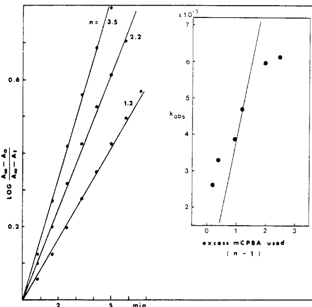
Figure 3. Plots of \log(A - A_0)/(A - A_i) at 415 nm vs time for the formation of 3 by the reaction of 1-OH with n equiv of mCPBA in methylene chloride at -48 \pm 0.5^\circ\text{C} . Inset: Effect of acid: ( ) observed; (—) calculated by eq 3, (...) calculated by eq 9.
