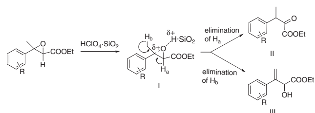
Scheme 2. Mechanism of the isomerization of glycidic esters.
