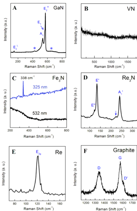
Figure 3. Raman spectra of the synthetic products resulting from HPSSM reactions between AMO and BN. (A) Hexagonal GaN. (B) Cubic VN. (C) Hexagonal \text{Fe}_3\text{N} . (D) Hexagonal \text{Re}_3\text{N} . (E) Hexagonal metal Re. (F) Nanosized hexagonal graphite. The Raman active modes are indexed. The 532 and 325 nm laser power is \sim 10 and \sim 15 mW, respectively.
