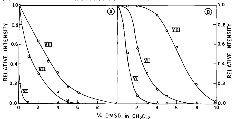
Fig. 3. Relative intensity of the amide-I C=O stretching band related to strongly self-associated molecules in the IR spectra of the hexa-, hepta-, and octapeptides VI , VII , and VIII , respectively, of series A (OChocb peptides) and series B (OBzl peptides) in CH_2Cl_2 /DMSO as a function of increasing percentages of DMSO. Peptide concentration is 10^{-2}M .
