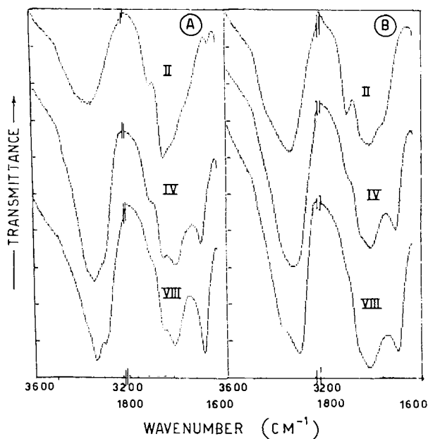
Fig. 1. Solid-state IR spectra in the 3600\text{--}3200\text{ cm}^{-1} and 1800\text{--}1600\text{ cm}^{-1} regions of the di-, tetra-, and octapeptides II , IV , and VIII , respectively with the OChocb ( A ) and the OBzl ( B ) substituent at the C-terminus
