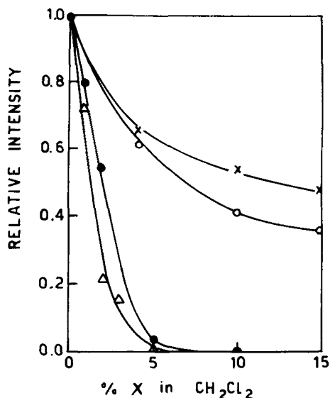
Fig. 4. Relative intensity of the amide-I C=O stretching band related to strongly self-associated molecules in the IR spectra of octapeptides VIII A in CH_2Cl_2 /X mixtures as a function of increasing percentages of X. X: HMPTA \Delta , DMSO \bullet , trimethyl phosphate \circ , and sulfolane \times . Peptide concentration is 10^{-3}M .
