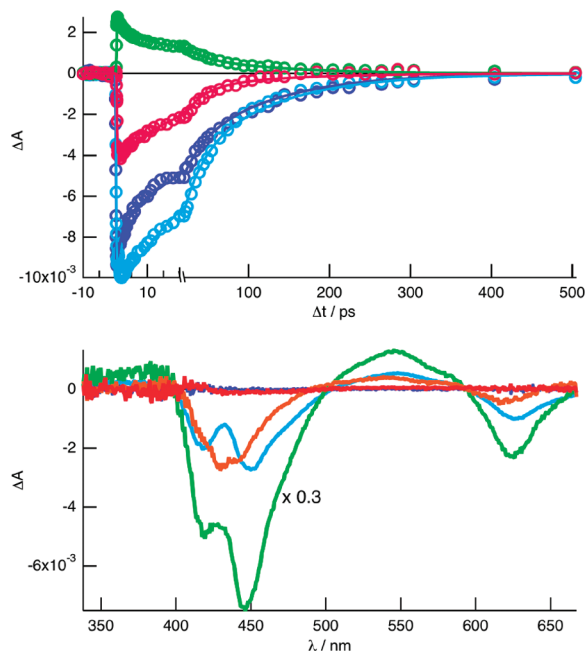
Figure 8. Transient spectra of dyad 11 in dichloromethane for AuP excitation at 690 nm. (Top) Dark blue, 420 nm; light blue, 450 nm; green, 545 nm; red, 630 nm. (Bottom) Dark blue, −10 ps; light blue, 5 ps; green, 20 ps; orange, 100 ps; red, 2000 ps. The double-peak feature in the Soret band disappears within about 10 ps and is likely not related to the charge-shift process (see text). Note that the 5 ps spectrum has been scaled by a factor of 0.3.
