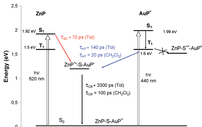
Scheme 3. Photophysical Behavior of Dyad 11
