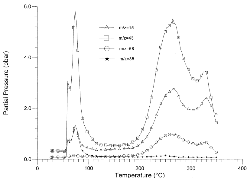
Fig. 5. TPRD profiles of [\text{Pd}(\text{acac})_2]/\text{MgO}^{\text{air}} .
