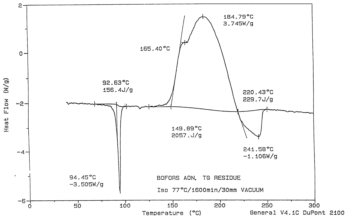
Fig. 18. DSC curve of BOFORS ADN TG residue (77°C) in nitrogen at 5°C/min.
