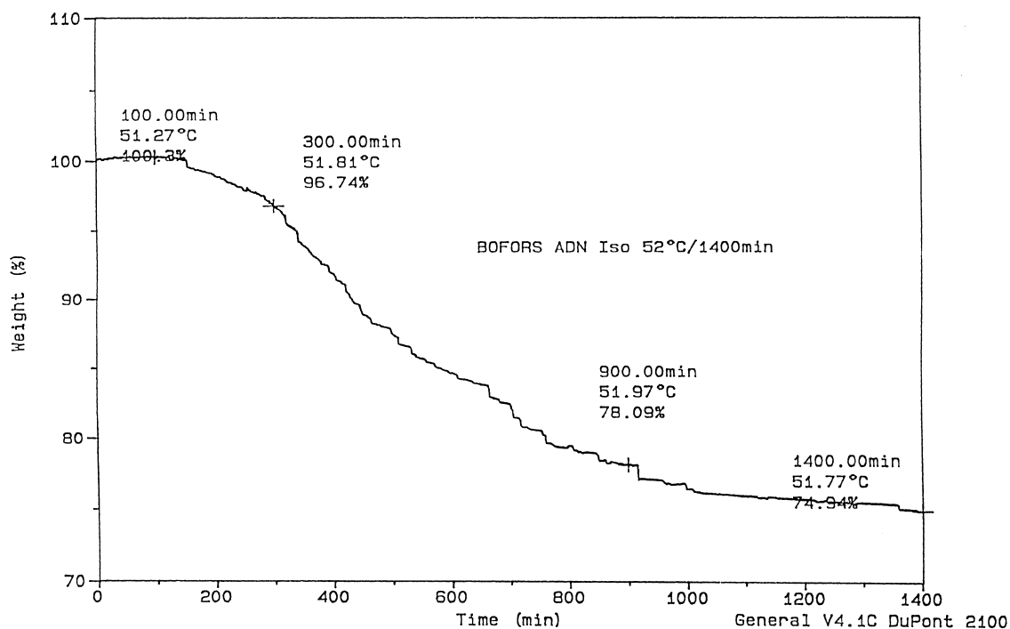
Fig. 13. Isothermal TG curve of BOFORS ADN in 35 mm vacuum at 52°C.
