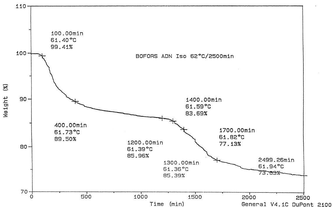
Fig. 14. Isothermal TG curve of BOFORS ADN in 35 mm vacuum at 62°C.
