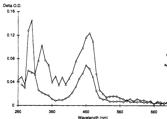
Figure 1. Transient spectra obtained after irradiating DMA with thymine dimer (diamonds) and dimethylthymine dimer (triangles) in pH 12 aqueous solution. Time is 3.0 \pm 0.2 \mu\text{s} following the laser pulse.
