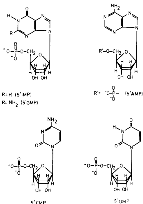
Fig. 1. Nucleotide structures and abbreviations used.
