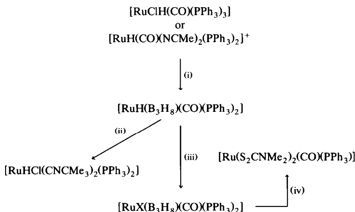
Scheme 1. (i) \text{NMe}_4[\text{B}_3\text{H}_8] ; (ii) \text{CNCMe}_3 ; (iii) \text{X-NC}_4\text{H}_4\text{O}_2 , \text{X} = \text{Cl}, \text{Br}, \text{I} ; (iv) \text{NaS}_2\text{CNMe}_2 .
