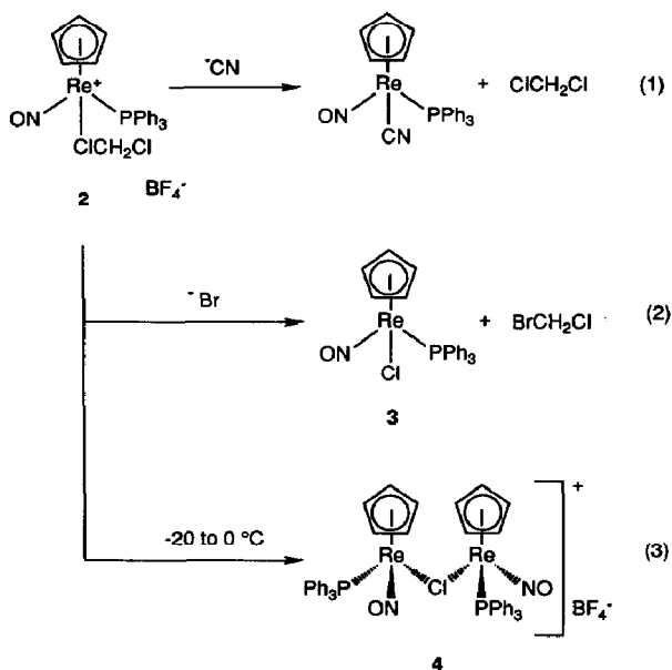
Scheme 1. Representative reactions of dichloromethane complex [(\eta^5\text{-C}_5\text{H}_5)\text{Re}(\text{NO})(\text{PPh}_3)(\text{ClCH}_2\text{Cl})]^+\text{BF}_4^- ( 2 ): (1) substitution at rhenium; (2) substitution at carbon; (3) thermal decomposition.
