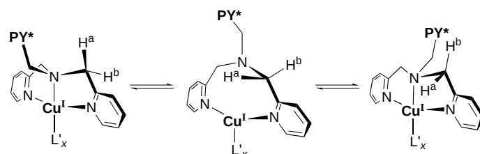
Scheme 3. Possible mechanism for exchange of the diastereotopic methylene protons in the Cu I complexes, [Cu(L)(L')] z+ ( 6 : L = L 1 , 7 : L = H 2 L 2 ; L' = ancillary (solvent or Cl - ) ligand), involving dissociation and inversion of the amine group.
