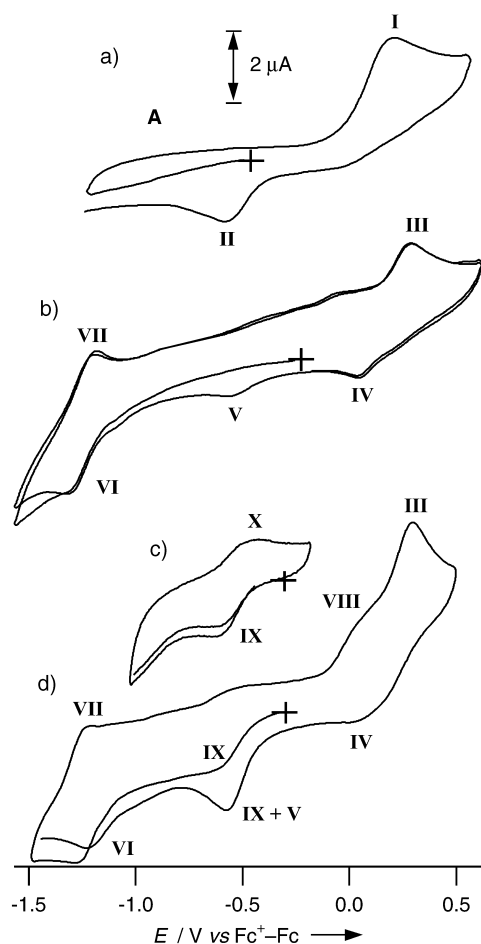
Figure 7. Cyclic voltammograms for: a) \text{H}_2\text{L}^2 ; b) [\text{Cu}(\text{HL}^2)]\text{PF}_6 ( 5 ); c and d) [\text{Cu}(\text{H}_2\text{L}^2)\text{Cl}_2] ( 3 ). Conditions: acetonitrile– 0.1\text{ M } [\text{Bu}_4\text{N}][\text{PF}_6] ; 295\text{ K} ; 1.0\text{ mm} Pt disk working electrode; scan rate = 100\text{ mV s}^{-1} .
