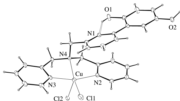
Figure 3. View of crystal structure of [\text{Cu}(\text{H}_2\text{L}^2)\text{Cl}_2] ( 3 ) (10% thermal ellipsoids shown). Key bond lengths [Å] and angles [°]: Cu–Cl1 2.225(1), Cu–Cl2 2.585(1), Cu–N2 2.011(3), Cu–N3 2.004(3), Cu–N4 2.052(3); Cl1–Cu–Cl2 106.3(1), Cl1–Cu–N2 97.5(1), Cl1–Cu–N3 97.8(1), Cl1–Cu–N4 160.4(1), Cl2–Cu–N2 92.9(1), Cl2–Cu–N3 91.5(1), Cl2–Cu–N4 93.3(1), N2–Cu–N3 162.3(1).
