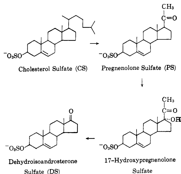
SCHEME I PROPOSED BIOSYNTHETIC PATHWAY INVOLVING STEROID SULFATES AS INTERMEDIATES
