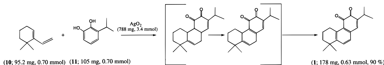
Figure 1. Reaction sequence of the ultrasound-promoted Diels–Alder cycloaddition as postulated by Lee et al. (1990) for the synthesis of miltirone (i.e., rosmariquinone; 1).
