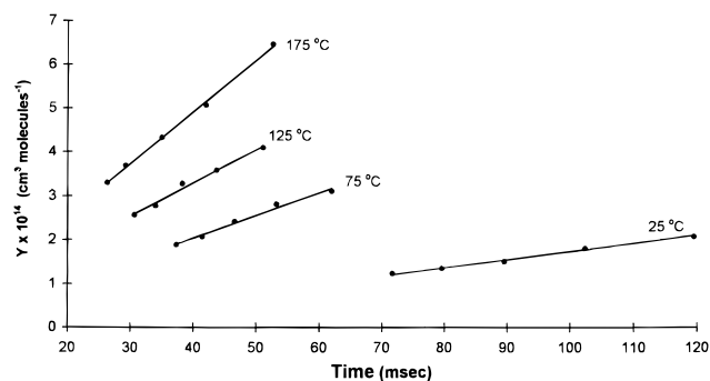
Figure 9. Extent of \text{Cl}^- -containing reactant ion loss determined by IMS measurements vs reaction time for several temperatures, plotted in the form of eq 17. The slopes of the lines thereby formed provide a phenomenological second-order rate constant, k_2' = k_2 + K_1k_1 , at each temperature. The concentrations of i\text{-PrBr} used at each temperature in order of increasing temperature are 7.3 \times 10^{14} , 4.14 \times 10^{13} , 5.89 \times 10^{13} , and 2.43 \times 10^{13} \text{ molecules cm}^{-3} .
