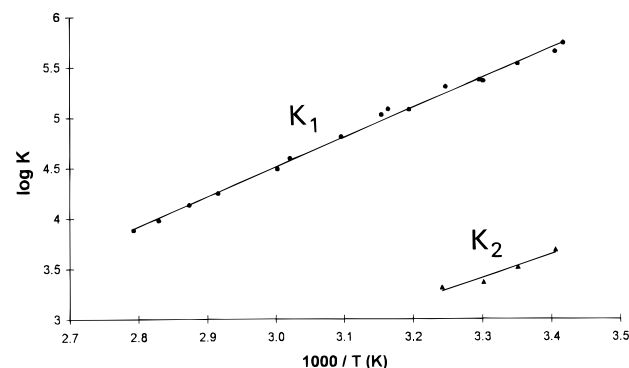
Figure 6. Van't Hoff plot of the equilibrium constants, K_1 , for the association of \text{Cl}^- with i\text{-PrBr} over the temperature range 20–85 °C, and for the equilibrium constants, K_2 , for the second-order clustering reaction, \text{Cl}^-(i\text{-PrBr}) + i\text{-PrBr} = \text{Cl}^-(i\text{-PrBr})_2 , over the temperature range 20–36 °C as determined by reaction-modified IMS measurements.
