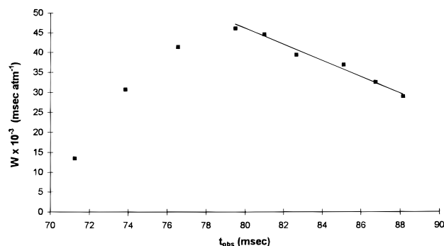
Figure 7. Drift time measurements for \text{Cl}^- -containing ions observed in reaction-modified IMS spectra under conditions of relatively high i\text{-PrBr} concentration at 35^\circ\text{C} , plotted in the form of eq 10 where W = (t_{\text{obs}} + t_{\text{obs}}K_1[i\text{-PrBr}] - t_0 - t_1K_1[i\text{-PrBr}])/K_1[i\text{-PrBr}]^2 . The slope of the straight line formed by t_{\text{obs}} measurements in excess of 80 ms provides a means of determining the equilibrium constant for second-order clustering, K_2 .
