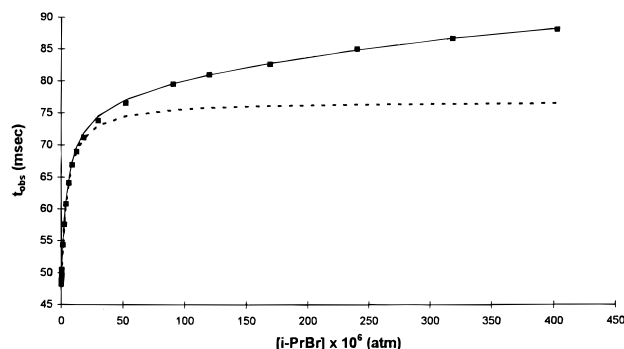
Figure 4. A typical measurement of the observed drift time, t_{\text{obs}} , for the \text{Cl}^- -containing ion packet versus the concentration of i\text{-PrBr} added to the drift gas at a relatively low temperature, 35 °C. The dashed line indicates the t_{\text{obs}} values expected if only first-order clustering with K_1 = 2.2 \times 10^5 \text{ atm}^{-1} were important, with K_2 assumed to be zero. The point at which the t_{\text{obs}} values begin to diverge from this dashed line indicates the onset of significant second-order clustering. The solid line indicates the t_{\text{obs}} values expected if both first- and second-order clustering are assumed to be important, with K_1 = 2.2 \times 10^5 \text{ atm}^{-1} and K_2 = 2.0 \times 10^3 \text{ atm}^{-1} . Excellent fit to all drift time measurements is then obtained.
