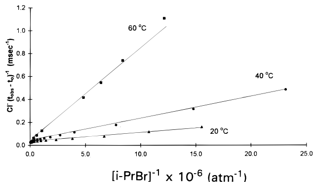
Figure 5. Changes in the drift time of the \text{Cl}^-/\text{Cl}^-(i\text{-PrBr}) ion packet as a function of i\text{-PrBr} concentration in the drift region, plotted in the form of eq 9. Equilibrium constants for the association of \text{Cl}^- with i\text{-PrBr} are determined from the intercepts and slopes of the least-squares lines thereby formed, as explained in the text.
