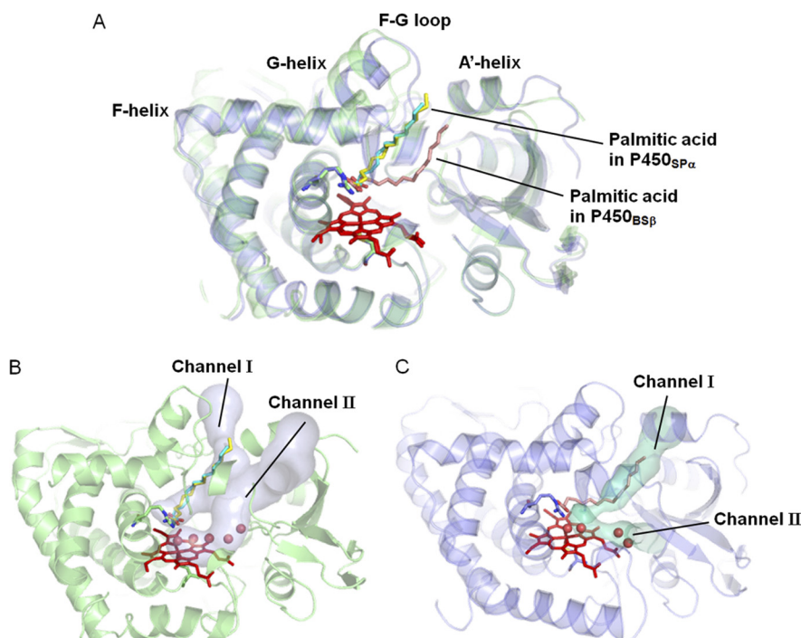
FIGURE 8. Overall structure of P450 SPα superposed on that of P450 BSβ . A, the superposition of the structures. The structures of P450 SPα and P450 BSβ are represented in green and blue , respectively. Heme is depicted as a red stick model . Palmitic acids in P450 SPα and P450 BSβ are represented as a yellow and cyan stick models and a pink stick model , respectively. B and C, substrate access channel location of P450 SPα (B) and P450 BSβ (C) calculated using CAVER (51) are shown as a light blue surface for P450 SPα and a cyan surface for P450 BSβ .
