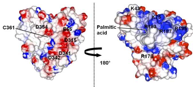
FIGURE 4. Electrostatic potential surface of P450 SPA . Electrostatic surfaces of P450 SPA were calculated using GRASP2 (49). The negatively charged surface is represented in red, and the positively charged surface is represented in blue. Palmitic acid is shown as a yellow stick model.
