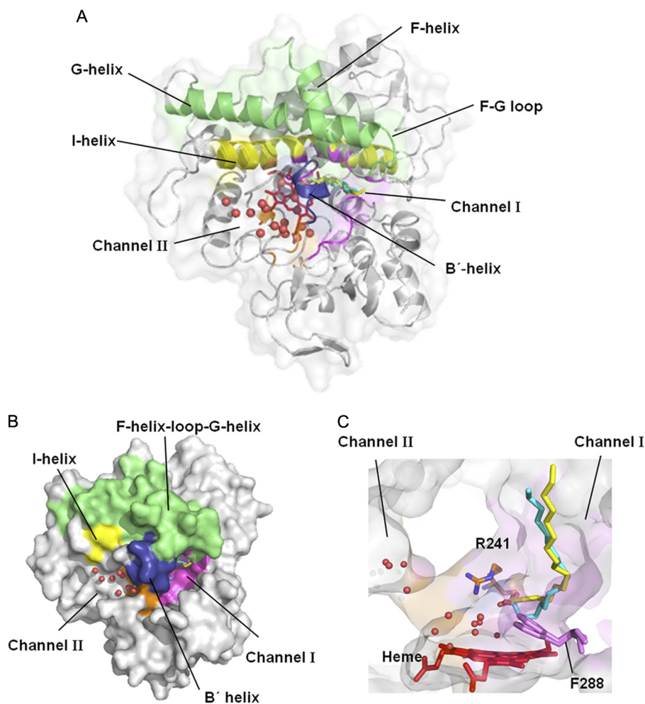
FIGURE 1. Overall structure of P450 SPα with palmitic acid. The B' helix and F helix-loop-G helix are colored in blue and green, respectively. Heme (red) and palmitic acid (yellow and cyan) are represented as stick models. The Channel I (magenta) and Channel II (orange) locations were calculated using CAVER (51). Water molecules in Channel II are represented as red spheres. A, the distal face of P450 SPα . B, surface model of P450 SPα . C, two channels of P450 SPα . Arg 241 (orange) and Phe 288 (purple) are labeled.
