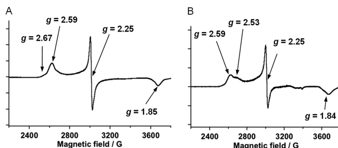
FIGURE 7. EPR spectra of P450 SPA recorded at 10 K. The spectra of P450 SPA in the absence (A) and presence of 120 μM of myristic acid (B) are shown. The concentrations of P450 SPA were 44 and 24 μM for the substrate-free form and for the myristic acid-bound form, respectively.
