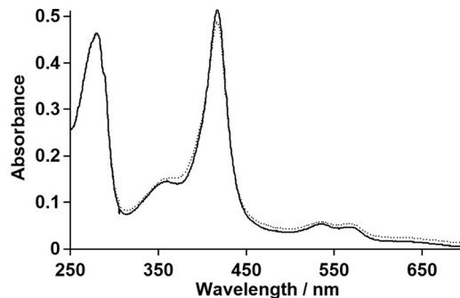
FIGURE 6. UV-visible absorption spectra of P450 SPA . The spectra of P450 SPA in 0.1 M potassium phosphate buffer (pH 7.0) containing 0.3 M KCl and 20% (v/v) glycerol in the absence (solid line) and presence of 120 μM of myristic acid (dotted line). The concentration of P450 SPA was 3.1 μM.
