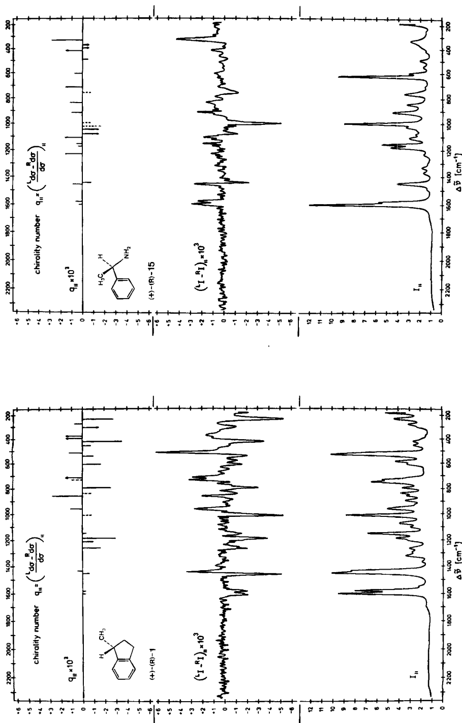
Fig. 1. The depolarized (measured in parallel polarization ||) Raman and circular difference Raman spectrum of (+)-(R)-1-methylindane (1; p = 1.00 ). The data are not corrected for instrument response. Slitwidth is 9 \text{ cm}^{-1} . I_n and q_n denote differential scattering cross sections for left and right circularly polarized light, respectively; see [27]. q -Numbers of strongly polarized bands are indicated by dashed lines; see text.
