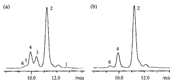
Figure 1. HPLC traces of chitooligosaccharide products from Chi 2 Nac-oxa (a) with ChiA1-Wt after 5 h and (b) with ChiA1-E204Q after 5 days; GlcNac(1), Chi 2 Nac(2), Chi 3 Nac(3), Chi 4 Nac(4), Chi 5 Nac(5), Chi 6 Nac(6). Sugar KS-802 column (Shodex, 8.0 × 300 mm) used for HPLC analysis (water eluent, 0.7 mL/min, 80 °C) with RI detector. A peak at 12.1 min is due to an impurity.
