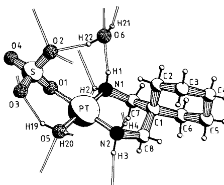
Fig. 3. PLUTO drawing of the asymmetric unit of \text{LPt}(\text{H}_2\text{O})\cdot\text{SO}_4\cdot\text{H}_2\text{O} ( 3 ) along with the adopted numbering scheme. The directions of the hydrogen bonds to neighbouring molecules have been indicated.
