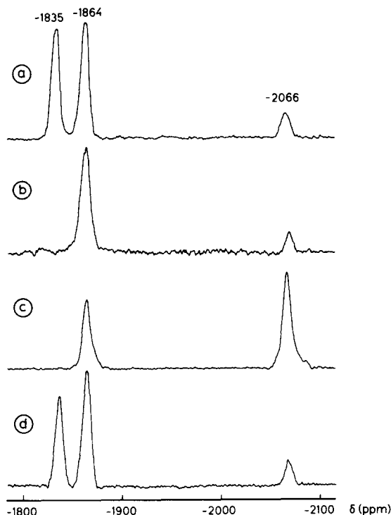
Fig. 2. Platinum-195 NMR spectra of various Pt(II) complexes in \text{D}_2\text{O} ; (a) \text{LPt}(\text{H}_2\text{O})\text{SO}_4 \cdot \text{H}_2\text{O} ( 3 ); (b) \text{LPt}(\text{NO}_3)_2 ( 4 ); (c) Solution of 4 containing 0.75 equivalents of \text{Cl}^- ; (d) Solution of 4 containing 1.1 equivalents of \text{SO}_4^{2-} .
