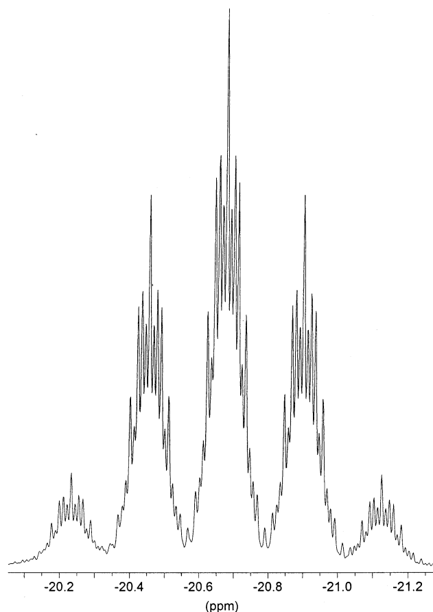
Figure 1. ^{11}\text{B} NMR spectrum of \text{K}[\text{B}(\text{CF}=\text{CF}_2)_4] in \text{CD}_3\text{CN} : an overlapping quintet of quintets of quintets ( ^2J_{\text{B,F}} = 21.5 , ^3J_{\text{B,F}} = 3.2 , ^4J_{\text{B,F}} = 2.2 Hz).
