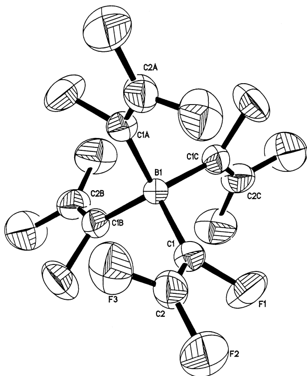
Figure 2. Anion in the [\text{NMe}_4][\text{B}(\text{CF}=\text{CF}_2)_4] salt. Displacement ellipsoids are drawn at the 40% probability level. Selected bond lengths (Å) and angles (deg): \text{B}-\text{C}(1) = 1.618(3) , \text{C}(1)-\text{C}(2) = 1.287(4) , \text{C}(1)-\text{F}(1) = 1.381(4) , \text{C}(2)-\text{F}(2) = 1.330(4) , \text{C}(2)-\text{F}(3) = 1.321(4) ; \text{C}(2)-\text{C}(1)-\text{B} = 132.1(3) , \text{C}(2)-\text{C}(1)-\text{F}(1) = 112.1(3) , \text{F}(1)-\text{C}(1)-\text{B} = 115.7(2) , \text{C}(1)-\text{C}(2)-\text{F}(2) = 126.3(4) , \text{C}(1)-\text{C}(2)-\text{F}(3) = 125.0(3) , \text{F}(2)-\text{C}(2)-\text{F}(3) = 108.7(3) , \text{C}(1)-\text{B}-\text{C}(1\text{A}) = 108.01(11) , \text{C}(1)-\text{B}-\text{C}(1\text{B}) = 112.4(2) .
