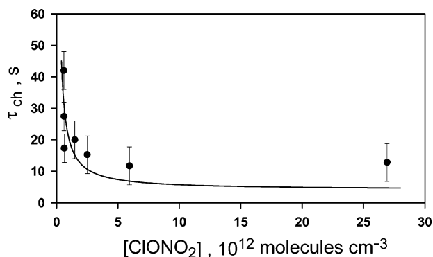
Figure 7. Dependence of the characteristic time \tau_{ch} on \text{ClONO}_2 concentration for the initial uptake of \text{ClONO}_2 on \text{NaCl} at T = 293 K. The symbols are experimental data. The solid curve shows approximation by \tau_{ch} = \tau_0(1 + n_{th}/[\text{ClONO}_2]) at \tau_0 = 4.1 \pm 0.6 s, n_{th} = 4 \times 10^{12} molecules \text{cm}^{-3} .
