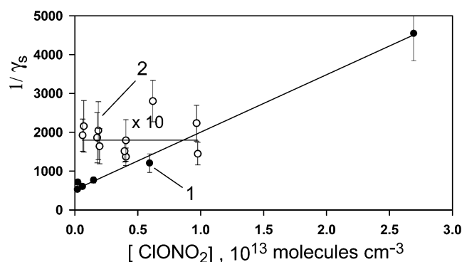
Figure 8. Dependence of the uptake coefficient \gamma_s on \text{ClONO}_2 concentration for steady-state uptake of \text{ClONO}_2 on \text{NaCl} . The symbols are experimental data at 293 K (1) and 387 K (2, on an enlarged scale). The solid lines show linear regressions by 1/\gamma_s(293 \text{ K}) = a_s + b_s[\text{ClONO}_2] at a_s = 521 \pm 61 , b_s = (14.8 \pm 0.6) \times 10^{-11} molecules ^{-1} \text{cm}^3 ; 1/\gamma_s(387 \text{ K}) = 179.6 \pm 21.5 .
