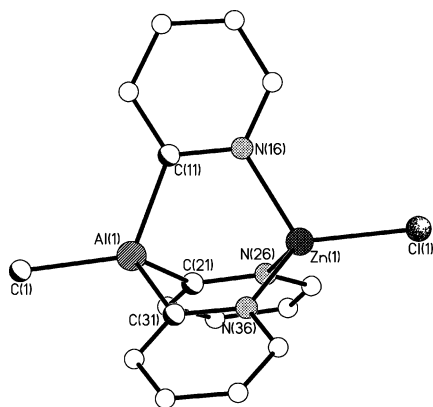
Figure 4. Structure of the monomeric molecule of [\text{MeAl}(\text{2-py})_3]\cdot\text{ZnCl} ( 4 ) illustrated by the 80% component of the disorder. H atoms have been omitted for clarity.
