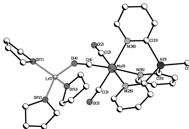
Figure 2. Structure of the trimetallic [\{\text{MeAl}(2\text{-py})_3\}\text{Mo}(\text{CO})_3\text{Li}(\text{THF})_3] ( 2 ). H atoms gave been omitted for clarity.
