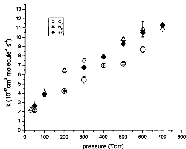
Figure 6. Second-order rate coefficients for reaction 1 in N 2 , O 2 , and air at 298 K.
