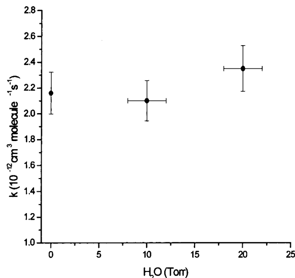
Figure 7. Second-order rate coefficients for reaction 1 as a function of the partial pressure of water vapor at a constant total pressure of 150 Torr in He buffer at 298 K.
