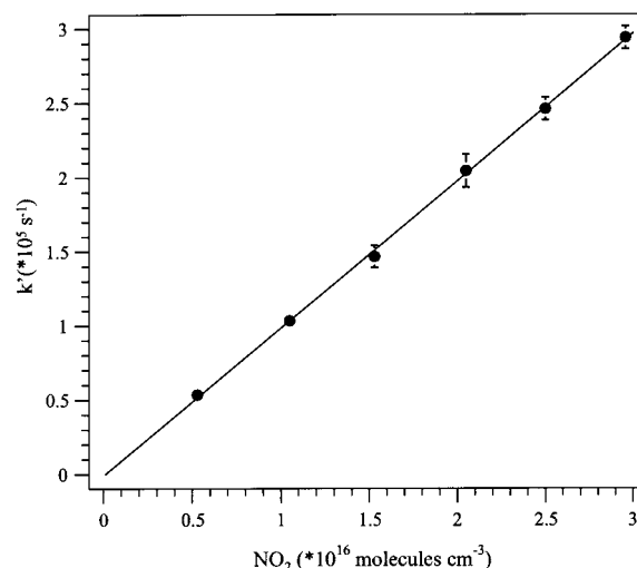
Figure 2. Plot of pseudo first-order rate versus [\text{NO}_2] in 600 Torr total pressure of N 2 at 295 K. The solid line shows the linear least-squares fit to the data and gives a second-order rate coefficient of k = (11.5 \pm 0.53) \times 10^{-12} cm 3 molecule -1 s -1 (error is 2\sigma ).
