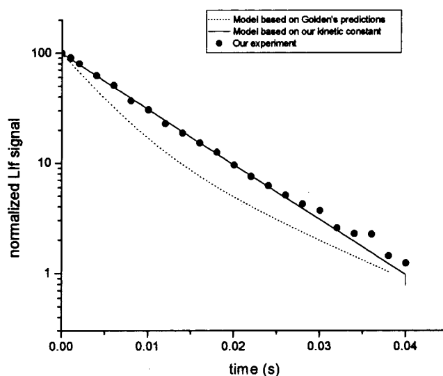
Figure 8. OH temporal profile in 600 Torr of He at 298 K in [NO 2 ] = 2.5 \times 10^{13} molecule/cm 3 . The straight line shows a least-squares fit to the data. The dotted line shows a simulation of the OH temporal profile obtained using the expressions proposed by Golden and Smith for the formation of nitric acid and the formation and decay of peroxyxynitrous acid.
