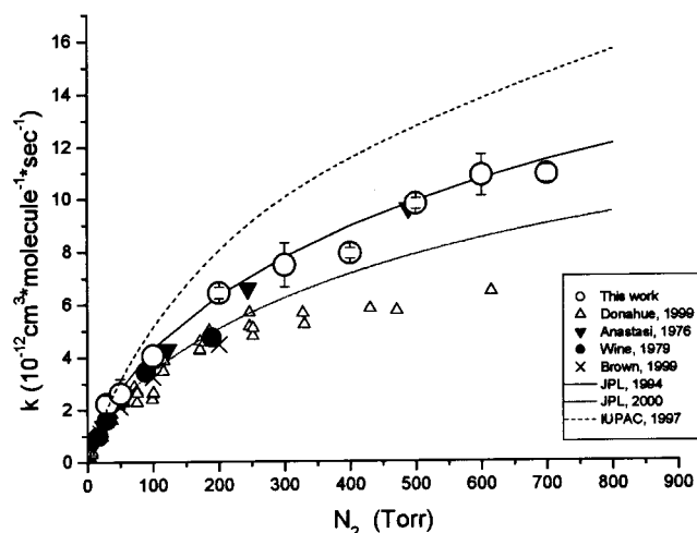
Figure 4. Second-order rate coefficients for reaction 1 in N 2 at 298 K, together with prior literature data. The solid and dotted lines show the JPL 2000, IUPAC 1997, and JPL 1994 recommendations.
