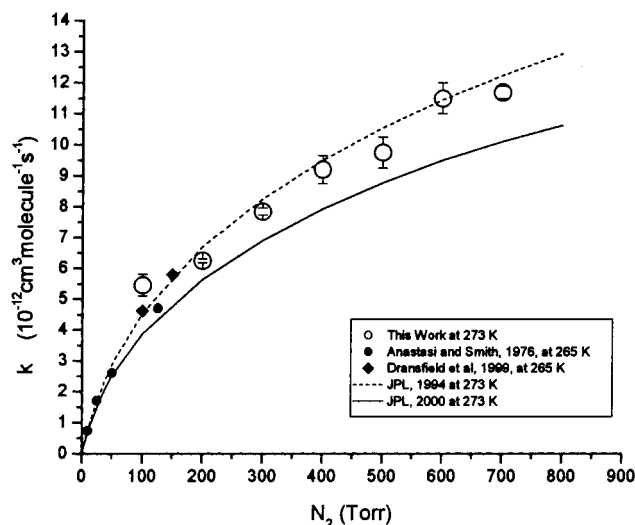
Figure 5. Second-order rate coefficients for reaction 1 in N 2 at 273 K, together with prior literature data. The solid and dotted lines show the JPL 2000 and JPL 1994 recommendations.
