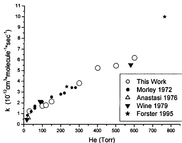
Figure 3. Second-order rate coefficients for reaction 1 in He at 298 K, together with prior literature data.
