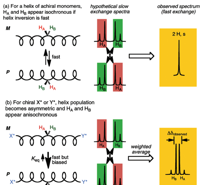
Figure 1. Detection of a helical preference by NMR spectroscopy in the fast-exchange regime.
