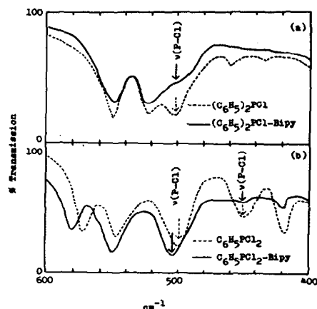
Figure 4. Infrared spectra of (C_6H_5)_2PCl , C_6H_5PCl_2 , and their 1:1 mixtures with 2,2'-bipyridyl in acetonitrile, 3 wt. %.
