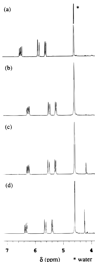
Figure 1. Proton chemical shifts for VS and ethylene binding to copper(I) in aqueous solution ( \text{D}_2\text{O} ): (a) VS (1.00 M) and \text{CF}_3\text{SO}_3\text{D} (0.10 M); (b) solution a and \text{CuOTf} (0.01 M); (c) solution b and ethylene (0.03 M); (d) solution b (0.15 M).
