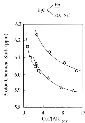
Figure 2. Chemical shift of the \text{H}_a proton in VS binding to copper(I) in aqueous solution containing \text{CF}_3\text{SO}_3\text{D} (0.10 M), \text{CuOTf} (0.01 M), and VS (0.06 M) at [\text{VS}]/[\text{Cu}] = 6 . Supplied gases: ethylene ( \circ ), 1,3-butadiene ( \square ), 1-butene ( \triangle ).
