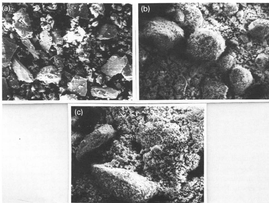
Fig. 2. Scanning electron micrographs of sphalerite: (a) as-received sample ( -74\ \mu\text{m} ); (b) mechanical activation t_G = 7.5\ \text{min} ; (c) mechanical activation t_G = 60\ \text{min} . Magnification, \times 200 .
