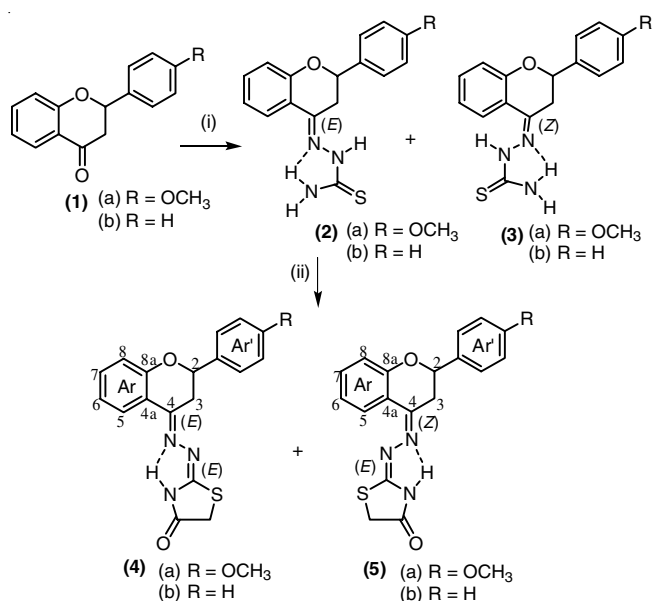
Fig. 1. Synthesis of 2 + 3 (i) 1 /H 2 N.NH.(C=S).NH 2 (molar ratio, 1:1.25), AcOH, absolute alcohol, reflux, 8 h. 4 + 5 (ii) 2 /Cl.CH 2 COOH/AcONa (molar ratio, 1:1.25:1.5), AcOH, reflux, 10 h
