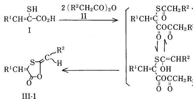
Chart 2. Possible Pathway for the Formation of Product III-1
