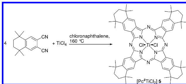
Scheme 2. Preparation of 5
