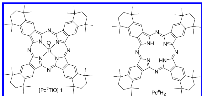
Figure 1. [\text{Pc}^\# \text{TiO}] 1 and the free ligand \text{Pc}^\# \text{H}_2 .
