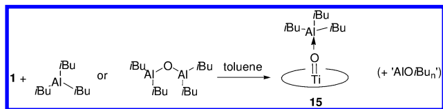
Scheme 6. Preparation of Lewis Acid Adduct 15
