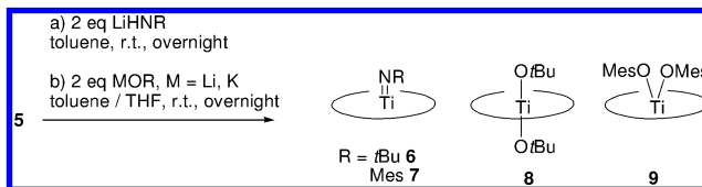
Scheme 3. Preparation of Axially Functionalized Titanium Phthalocyanines 6–9 via Salt Elimination a
