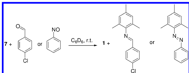
Scheme 7. Nitrene Transfer Reaction of 7
