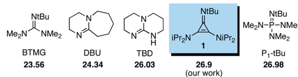
Figure 2. Basicity of cyclopropenimine 1 and several common strong organic bases. Bold numbers are pK_{BH^+} values in acetonitrile.
