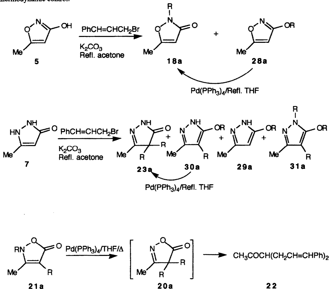
SCHEME IV
