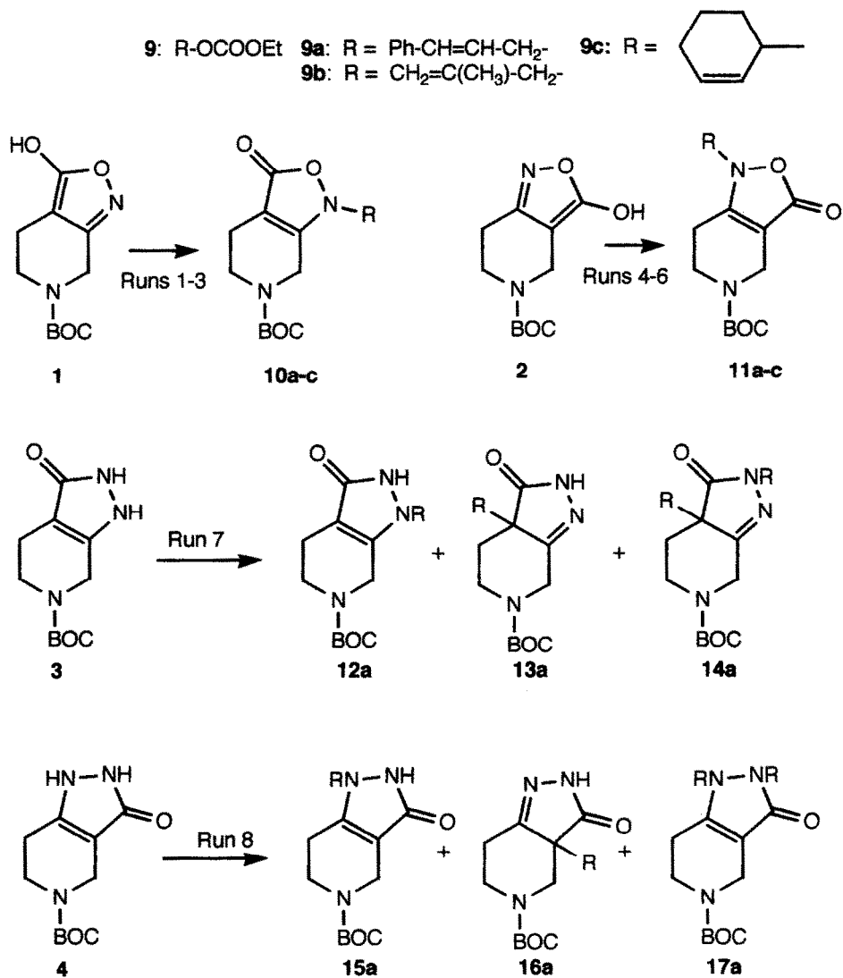
SCHEME II
