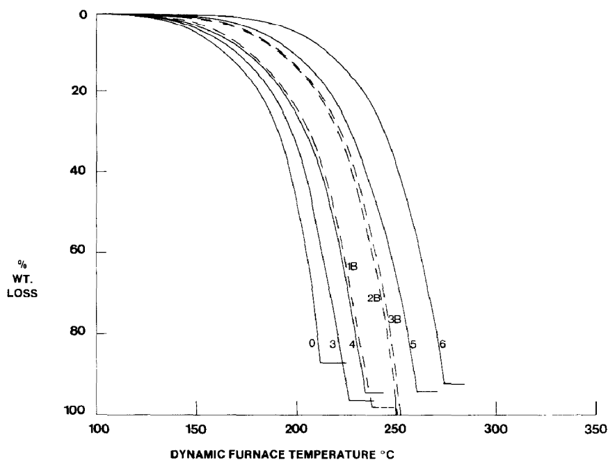
Fig. 2. Thermograms (TG) for aryltricarboxylchromium(0) complexes in argon. 0–6 and 1B, 2B and 3B identify the number of methyl and t -butyl substituents, respectively in the complex (see Experimental section for identification of the aryl ligands).
