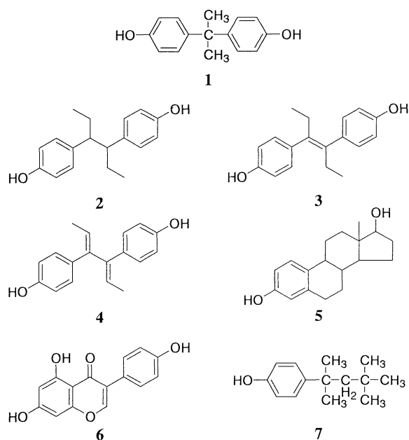
Figure 1. Structures of phenolic estrogenic and xenoestrogenic compounds: 1 , bisphenol A; 2 , hexestrol; 3 , diethylstilbestrol; 4 , dienestrol; 5 , 17 \beta -estradiol; 6 , genistein; 7 , p - t -octylphenol.
