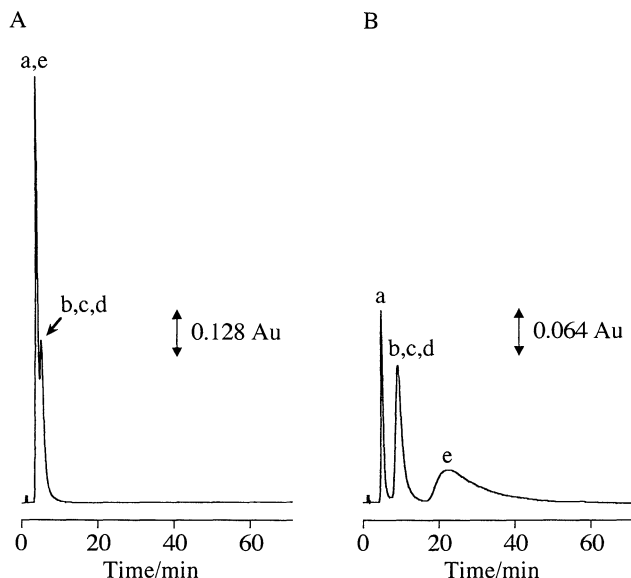
Figure 2. Separation of phenolic estrogenic and xenoestrogenic compounds on the non-imprinted polymer (A) and the MIP (B) for bisphenol A. Peak assignments: a, 17 \beta -estradiol ( 5 ); b, hexestrol ( 2 ); c, dienestrol ( 4 ); d, diethylstilbestrol ( 3 ); e, bisphenol A ( 1 ). HPLC conditions as in Table 2. Loaded amounts: 1 , 400 ng; 2 , 3 and 4 , 80 ng; 5 , 160 ng.
