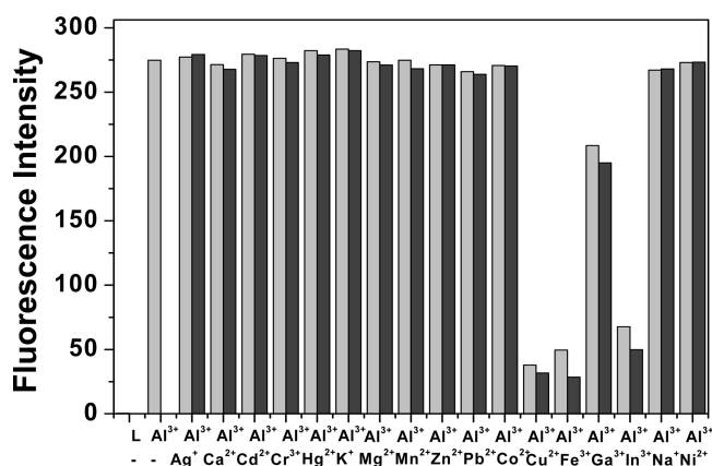
Figure 7. Relative fluorescence of PSI and its complexation with \text{Al}^{3+} in the presence of various metal ions. Response of PSI was included as controls. (Left to right) PSI alone (L corresponds to PSI), \text{PSI} + \text{Al}^{3+} , \text{PSI} + \text{Al}^{3+} + \text{Ag}^+ , \text{PSI} + \text{Al}^{3+} + \text{Ca}^{2+} , etc. Conditions: 1.0 \mu\text{M} of PSI, 12 equiv of \text{Al}^{3+} in the absence and presence of 12 (gray) and 24 equiv (black) of metal ions with ( \lambda_{\text{ex}} = 411 \text{ nm} ).
