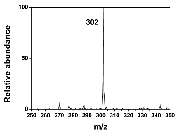
Figure 6. Positive-ion electrospray ionization mass spectrum of PSI upon addition of \text{Al}(\text{NO}_3)_3 (1 equiv) in \text{CH}_3\text{OH} .
