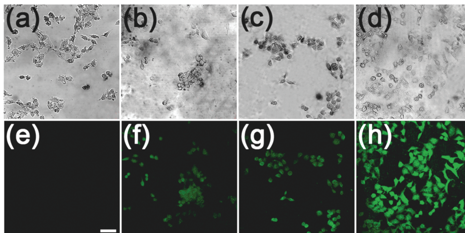
Figure 8. Representative fluorescence images of HeLa cells exposed to various concentrations of \text{Al}(\text{NO}_3)_3 with 10 \mu\text{M} PSI: (a and e) incubated with PSI only; (b and f) incubated with 1 \mu\text{M} \text{Al}(\text{NO}_3)_3 for 4 h and exposed with PSI; (c and g) incubated with 10 \mu\text{M} \text{Al}(\text{NO}_3)_3 for 4 h and exposed with PSI; (d and h) 100 \mu\text{M} \text{Al}(\text{NO}_3)_3 for 4 h and stained with PSI. (a–d) DIC images and (e–h) fluorescent images (excitation = 480 \text{ nm} , emission = 520 \text{ nm LP} ). Details are found in the Experimental Section. Scale bar represents 50 \mu\text{m} .
