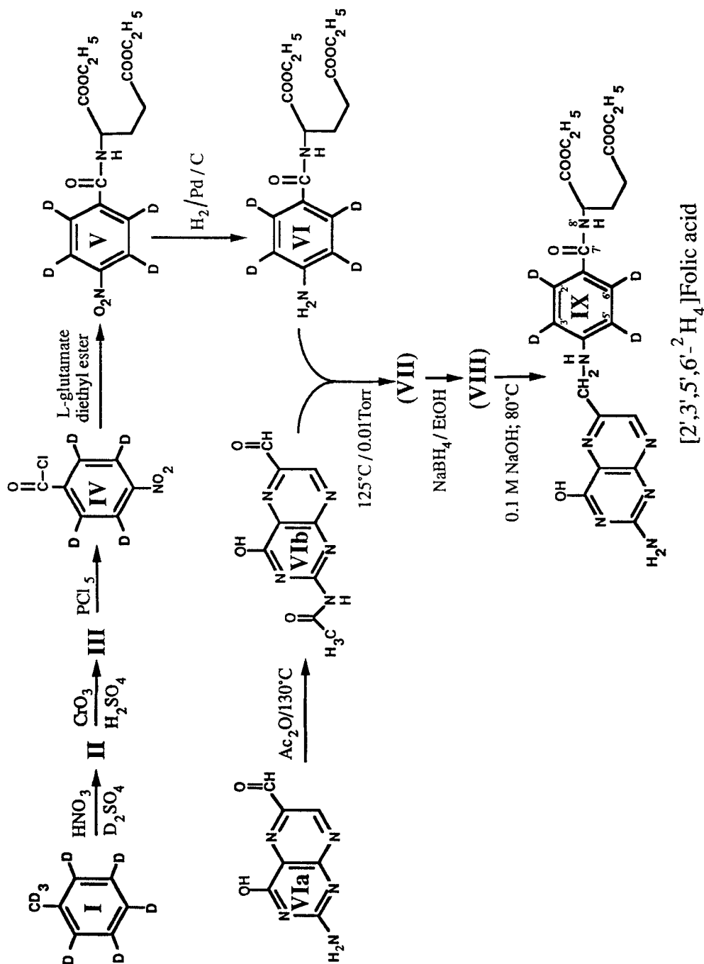
Figure 1. Scheme for synthesis of [2',3',5',6'- ^2\text{H}_4 ]folic acid. The key intermediate, VI , was prepared from toluene-d 8 and coupled to VIb .
