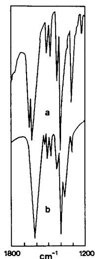
Fig. 2. IR spectra (1800–1200 cm -1 region) of powdered solid samples spread on NaCl disks. (a) [(phen)(Ph 3 P)Cu(O 2 COH)] (A); (b) [(phen)(Ph 3 P)Cu(O 2 COH)] (3).
