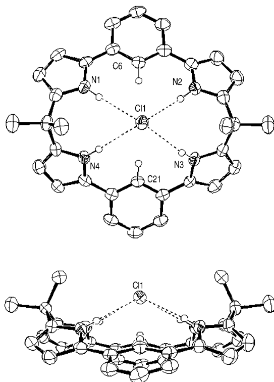
Figure 3. X-ray crystal structure of 9a ·Cl − (ORTEP, displacement ellipsoids scaled to the 50% probability level; some hydrogen atoms have been removed for clarity). Top: top view; bottom: side view. Dashed lines are indicative of N–H...Cl − hydrogen bonds.
