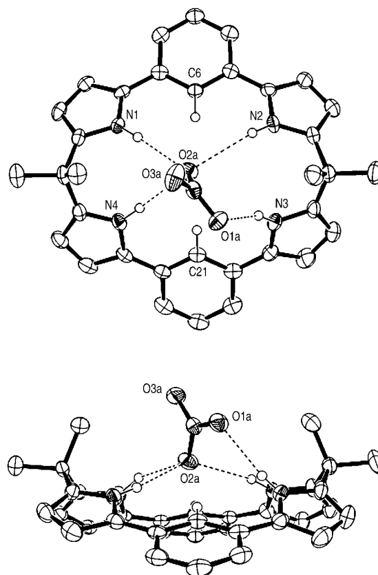
Figure 4. X-ray crystal structure of 9a ·NO 3 − (ORTEP, displacement ellipsoids scaled to the 50% probability level; some hydrogen atoms have been removed for clarity). Top: top view; bottom: side view. Dashed lines are indicative of N–H...O hydrogen bonds.
