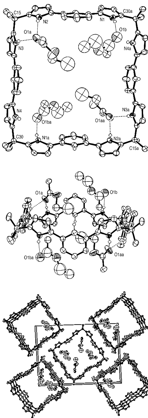
Figure 7. X-ray crystal structure of 11a ·( \text{C}_4\text{H}_8\text{O}_2 ) 4 (ORTEP, displacement ellipsoids scaled to the 30% probability level; some hydrogen atoms omitted for clarity). Top: top view; middle: side view; bottom: unit-cell packing diagram. Dashed lines are indicative of N–H···O hydrogen bonds. The ethyl acetate molecules with atoms O1b, O1ba are hydrogen bonded to a second macrocycle related by a b axis translation.
