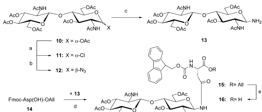
Scheme 3. Synthesis of chitobiosyl asparagine building block 16 . a) sat. HCl in acetyl chloride, RT, 48 h, 82 %; b) NaN 3 (3.1 equiv), aliquat 336 (1.0 equiv), CHCl 3 /H 2 O, RT, 42 h, 70 %; c) H 2 , raney-nickel, dioxane/EtOH, RT, 3 h, quant.; d) TBTU (1.0 equiv), HOBt (1.0 equiv), DIPEA (2.0 equiv), DMF, RT, 40 h, 76 %; e) [Pd(PPh 3 ) 4 ] (0.06 equiv), sodium- p -toluenesulfonate (1.3 equiv), THF/MeOH, RT, 70 min, 57 %.
