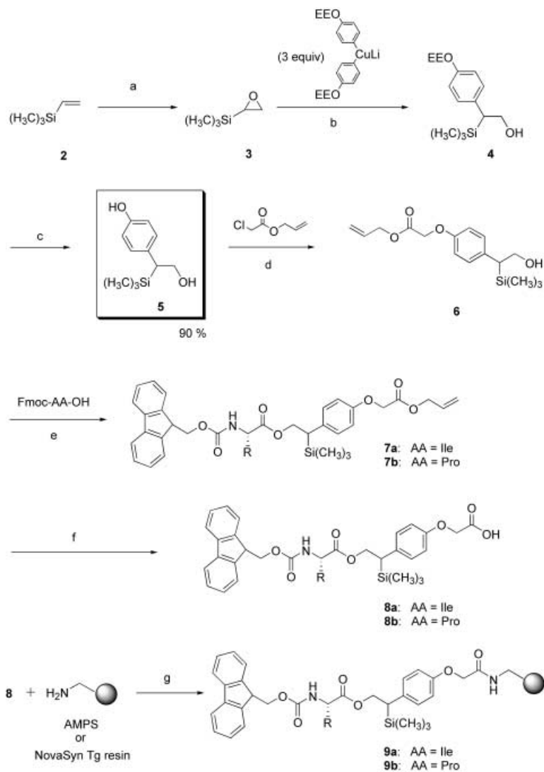
Scheme 2. Synthesis of the PTMSEL-linker and loading of the resin. a) m CPBA (1.0 equiv), CHCl 3 , RT, 60 h, 74%; b) lithium [di( p -1-ethoxyethoxy)-phenyl]cuprate (3.0 equiv), diethyl ether, −50°C, 5 h → −20°C, 14 h, 85%; c) PPTS (0.03 equiv), MeOH, RT, 2 h, 90%; d) allyl chloroacetate (1.9 equiv), K 2 CO 3 , KI, acetone, RT, 38 h, 78%; e) Fmoc-AA-OH (1.1 equiv), DCC (1.2 equiv), DMAP (0.06 equiv), CH 2 Cl 2 , 0°C, 4 h, > 90%; f) [Pd(PPh 3 ) 4 ] (0.06 equiv), p -toluenesulfonate (1.3 equiv), THF/MeOH, RT, 90 min, quant.; g) TBTU (1.0 equiv), HOBT (1.0 equiv), NMM (2.0 equiv), CH 2 Cl 2 /DMF, RT, 18 h.
