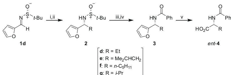
Scheme 2. Reagents and conditions: (i) Method A: \text{RMgBr} (1.5 equiv), \text{Me}_2\text{Zn} (1.7 equiv), THF, -78^\circ\text{C} . Method B: \text{RMgBr} (1.3 equiv), \text{Me}_2\text{Zn} (0.15 equiv), THF, -78^\circ\text{C} ; (ii) \text{NH}_4\text{Cl} (aq); (iii) \text{HCl} , \text{MeOH} ; (iv) \text{PhCOCl} (2.8 equiv), \text{Et}_3\text{N} (2.8 equiv), \text{CHCl}_3 , 0 – 20^\circ\text{C} . (v) \text{RuCl}_3 \cdot x\text{H}_2\text{O} (5 mol %), \text{NaIO}_4 (6 equiv), \text{MeCN:H}_2\text{O:CCl}_4 (1.5:1.5:1), 20^\circ\text{C} .
