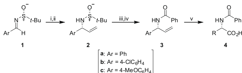
Scheme 1. Reagents and conditions: (i) Method A: \text{CH}_2=\text{CHMgBr} (1.5 equiv for 1a–b , 2.25 equiv for 1c ), \text{Me}_2\text{Zn} (1.7 equiv for 1a–b , 2.5 equiv for 1c ), THF, -78^\circ\text{C} ; Method B: \text{CH}_2=\text{CHMgBr} (1.3 equiv), \text{Me}_2\text{Zn} (0.15 equiv), THF, -78^\circ\text{C} ; (ii) \text{NH}_4\text{Cl} (aq); (iii) \text{HCl} , \text{MeOH} ; (iv) \text{PhCOCl} (2.8 equiv), \text{Et}_3\text{N} (2.8 equiv), \text{CHCl}_3 , 0 – 20^\circ\text{C} ; (v) \text{RuCl}_3 \cdot x\text{H}_2\text{O} (1.2 mol %), \text{NaIO}_4 (4 equiv), \text{MeCN:H}_2\text{O:CCl}_4 (1:1.5:1), 20^\circ\text{C} .
