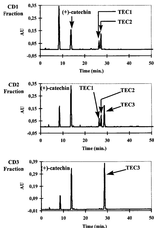
Figure 7. HPLC chromatograms recorded at 280 nm of CD1, CD2, and ED3 fraction thiolysis.
