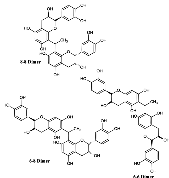
Figure 3. General structure of (–)-epicatechin–ethyl dimers.
